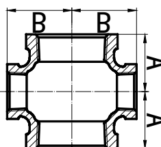
Reducing Cross
