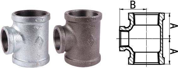
Reducing Tee
