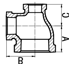
Pitcher Tee
